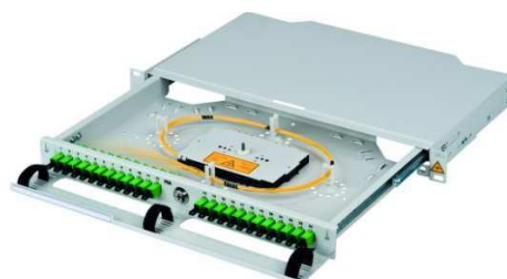
Equipped of PSP-T patch panel
